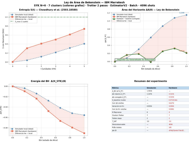
FIG. 9. Experiment 6 — Bekenstein area law on ibm_marrakesh . Top left: S(t) replicating Chowdhury et al. Top right: \Delta A(\theta) simulator vs. hardware (baseline-corrected): the simulation satisfies \Delta A \geq 0 ; the hardware does not resolve \Delta A(\theta) above noise. Bottom left: \Delta\langle H_{\text{SYK}} \rangle vs. \theta . Bottom right: summary table with Job ID.
