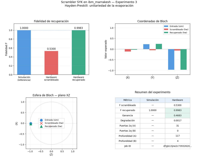
FIG. 6. Experiment 3 — Hayden-Preskill on ibm_marrakesh . Top left: recovery fidelity F_{\text{scr}} = 0.530 , F_{\text{rec}} = 0.9983 . Top right: Bloch coordinates before/after scrambling/recovery. Bottom left: Bloch sphere XZ plane. Bottom right: summary table.
